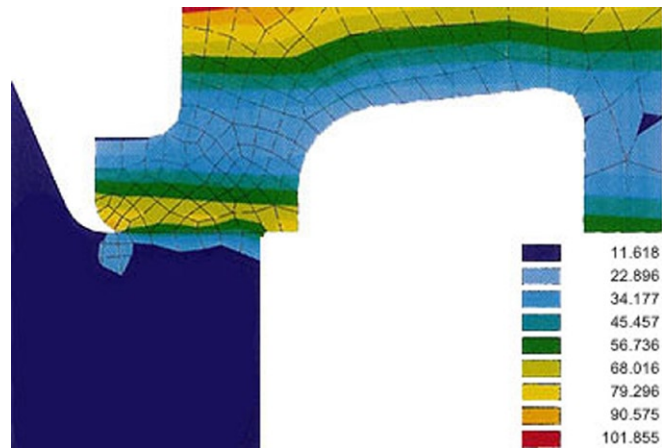
IPP DELTAFLEX® flange, Units are Mpa (N/mm 2 )
