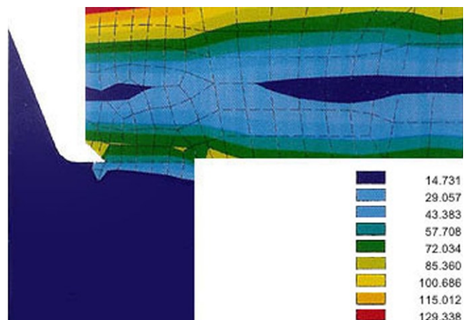
Conventional Steel Flange, Units are Mpa (N/mm 2 )
